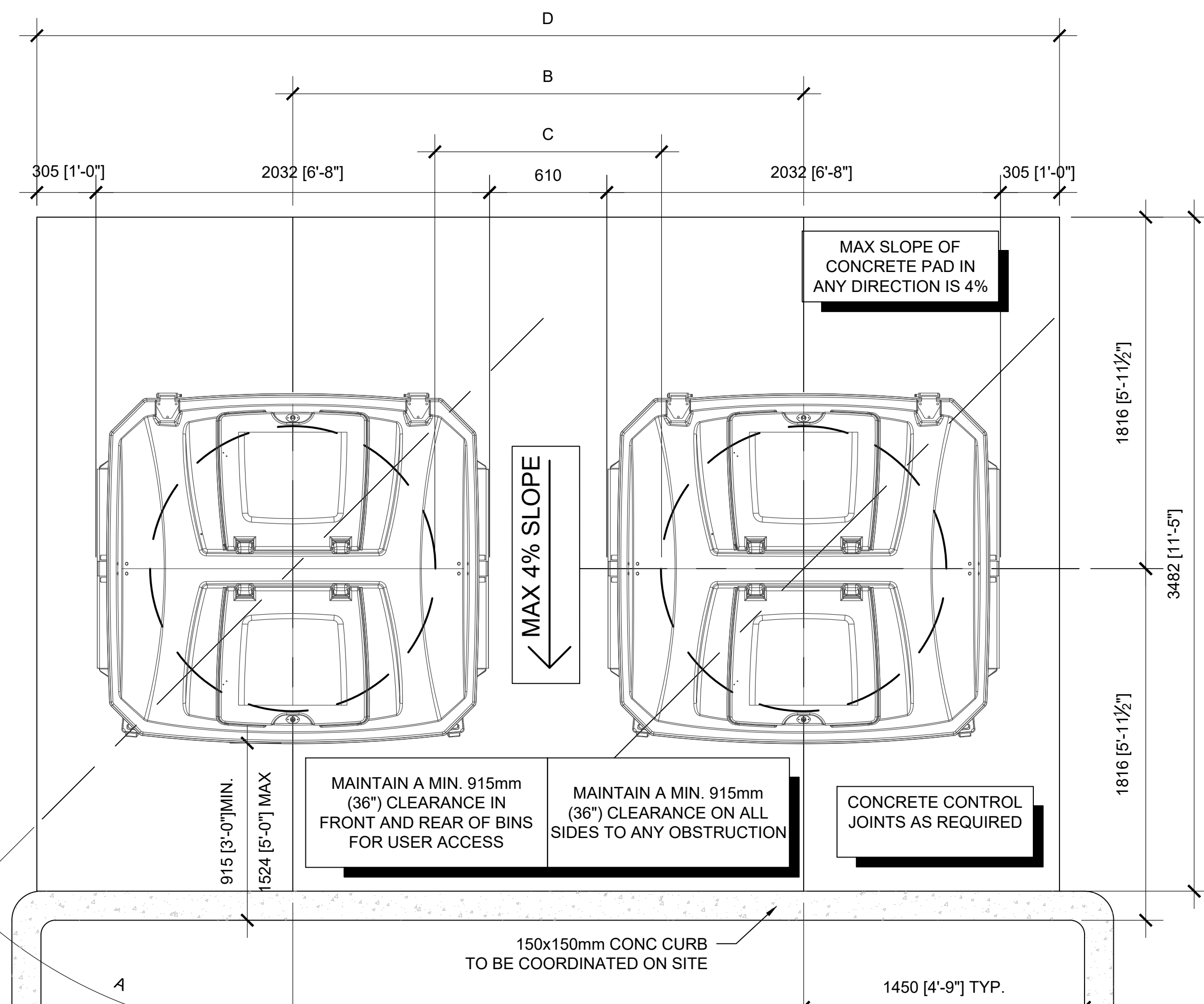
3 A1 TYPICAL PLAN VIEW W/O BOLLARDS 1:20
