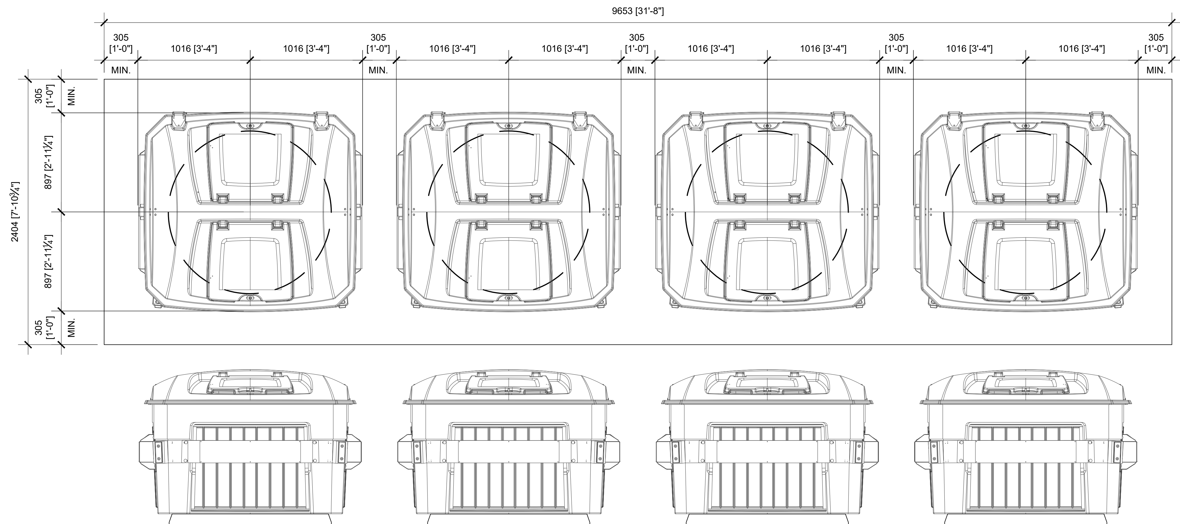
3 A3 TYP. PLAN & ELEV VIEW - 4 BINS 1:20
