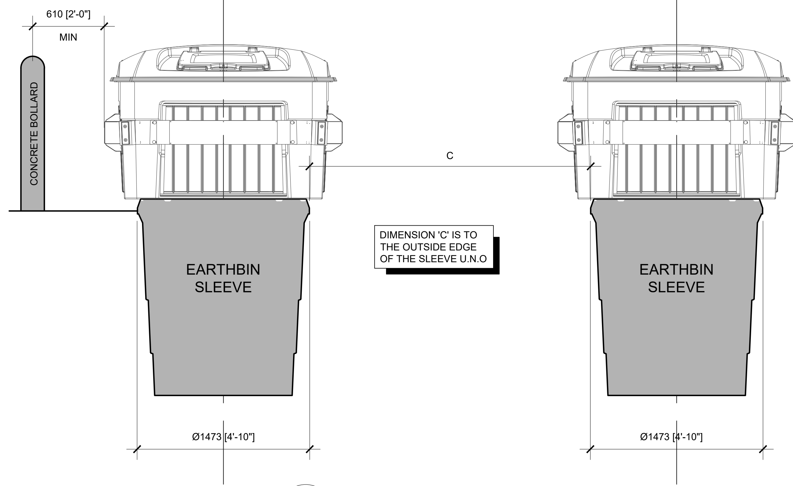
2 A1 ELEVATION VIEW OF BINS 1:20
