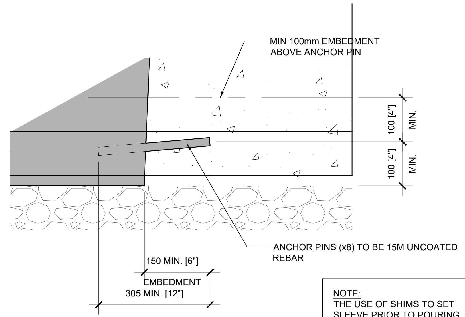
3 A2 1:5 SLEEVE DETAIL B
