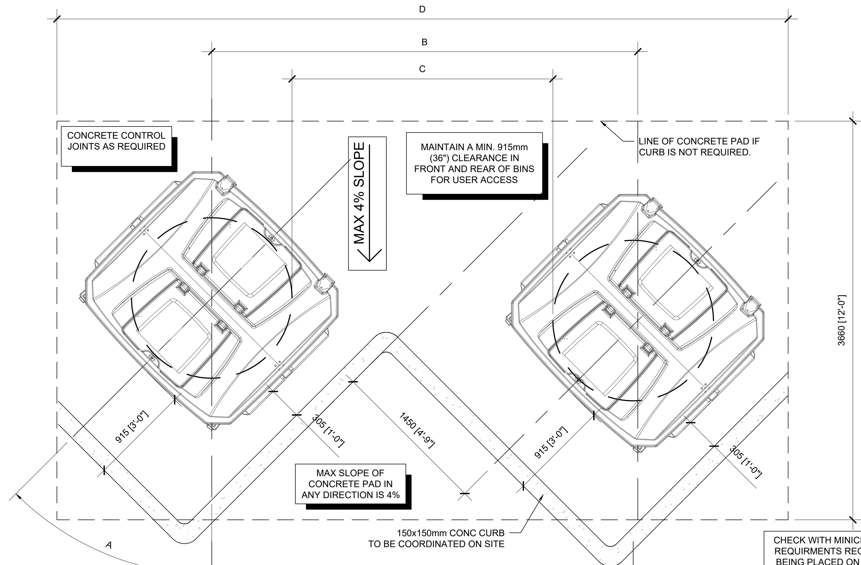
1 A1 ANGLED PLAN VIEW W/O BOLLARDS 1:20
