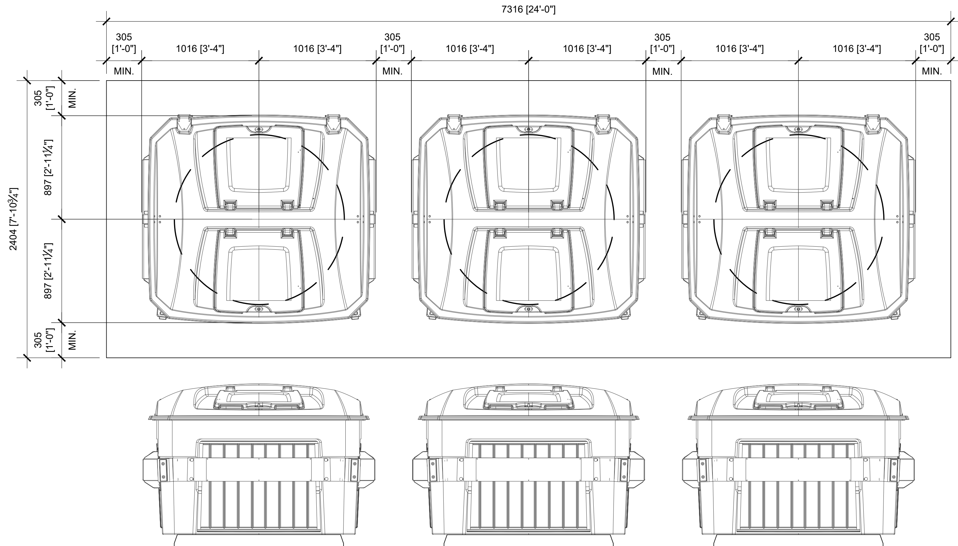
2 A3 TYP. PLAN & ELEV VIEW - 3 BINS 1:20
