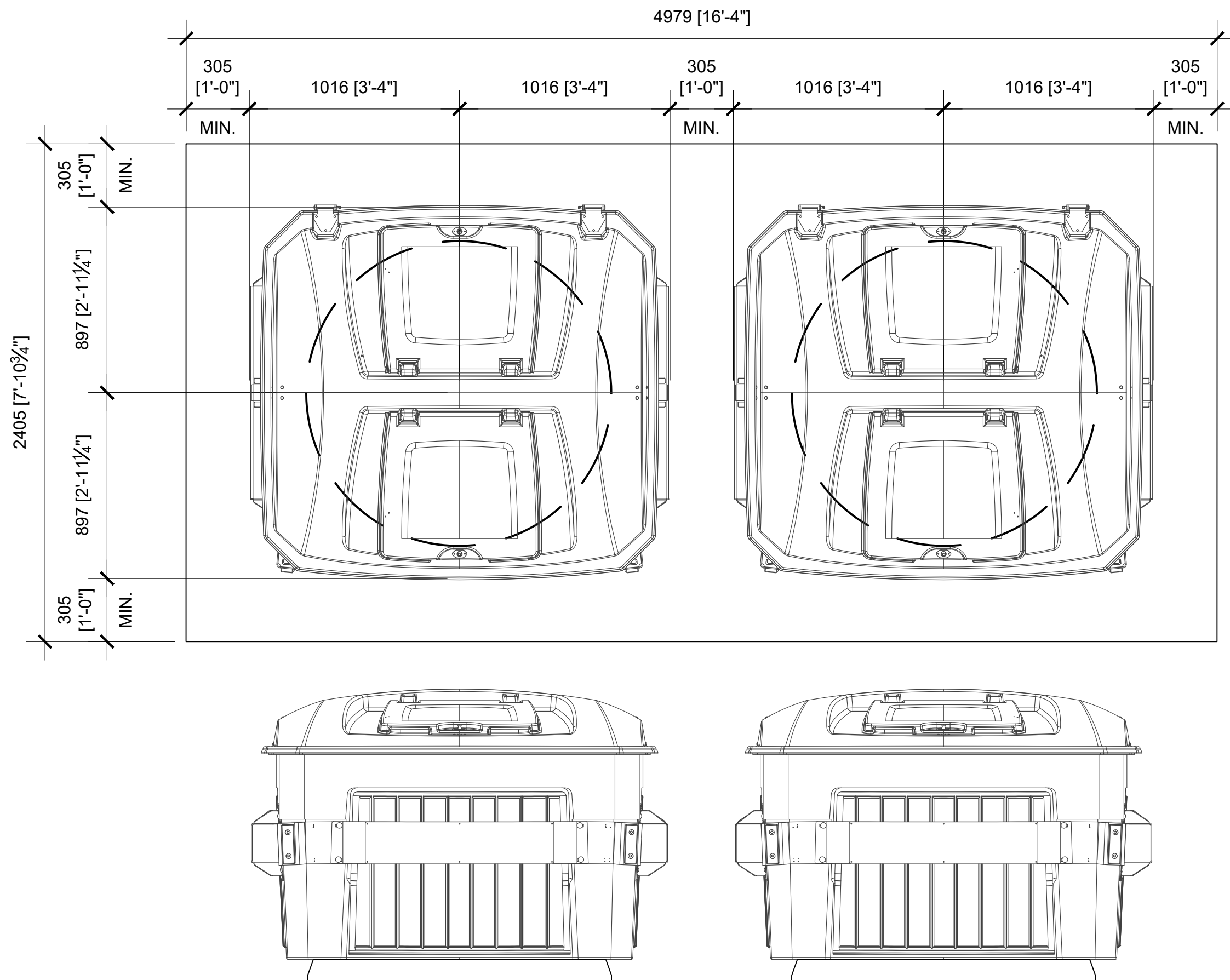
1 A3 TYP. PLAN & ELEV VIEW - 2 BINS 1:20
