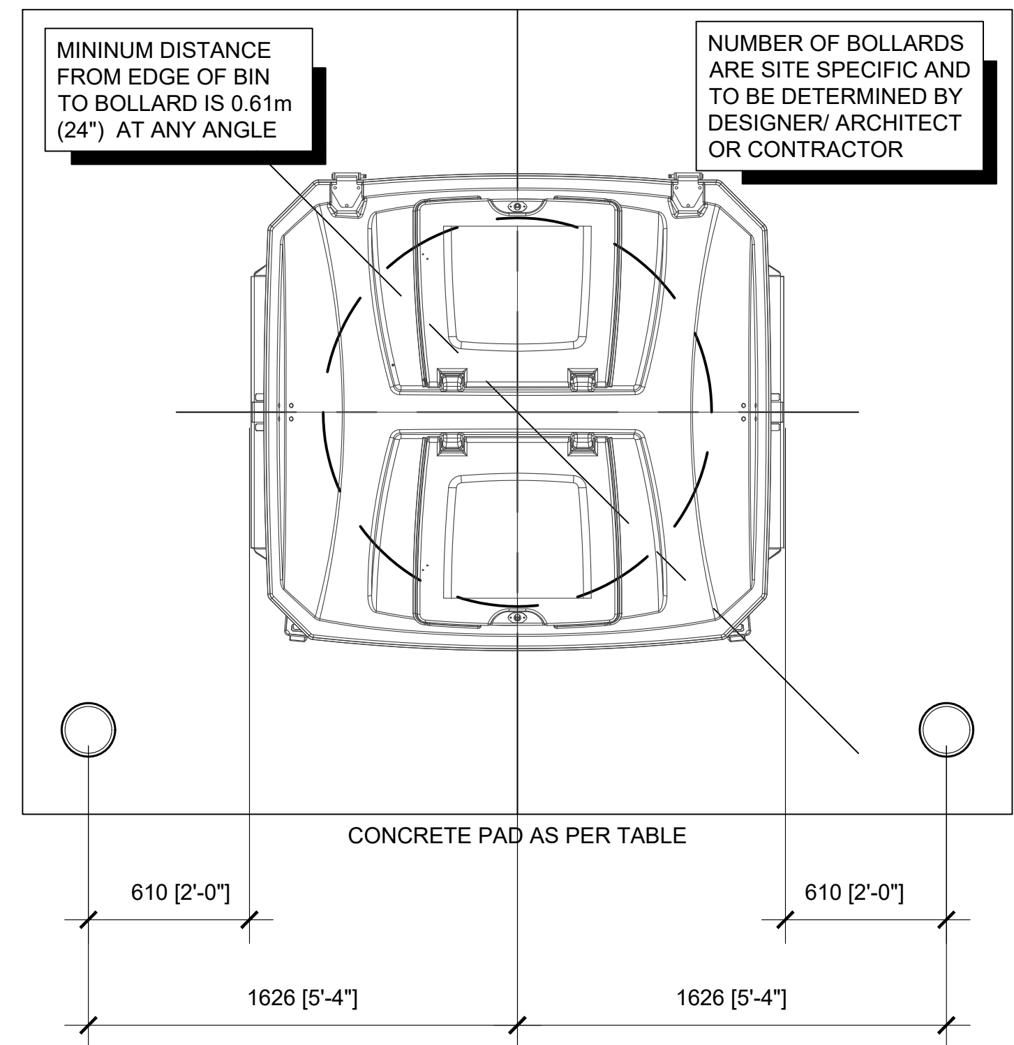
4 A1 OPTIONAL BOLLARD PLACEMENT 1:20
